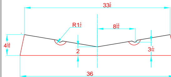
TRANSVERSAL SECTION "A" SECCION TRANSVERSAL "A"
